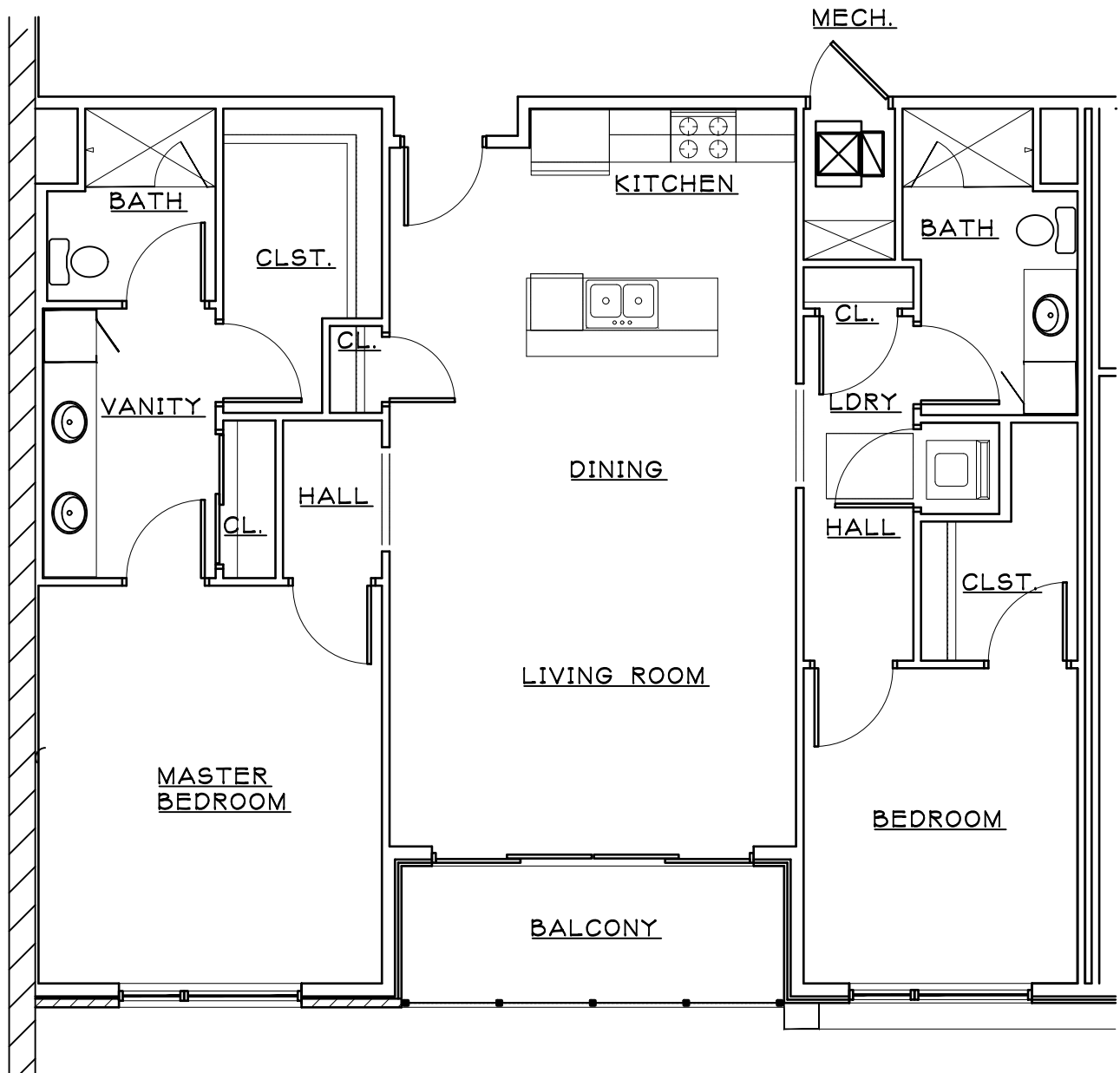
UNITS 201, 301 & 401 (1321 SQ.FT.)
